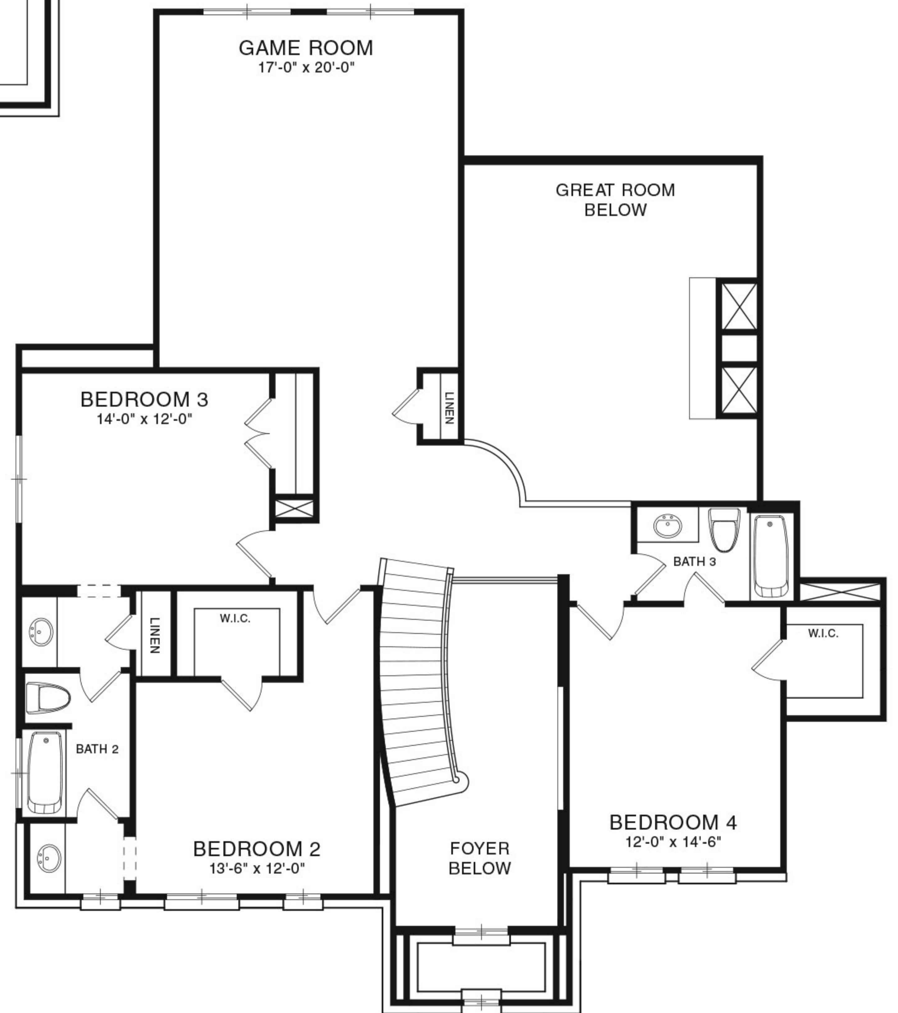
SECOND FLOOR PLAN STYLE A
