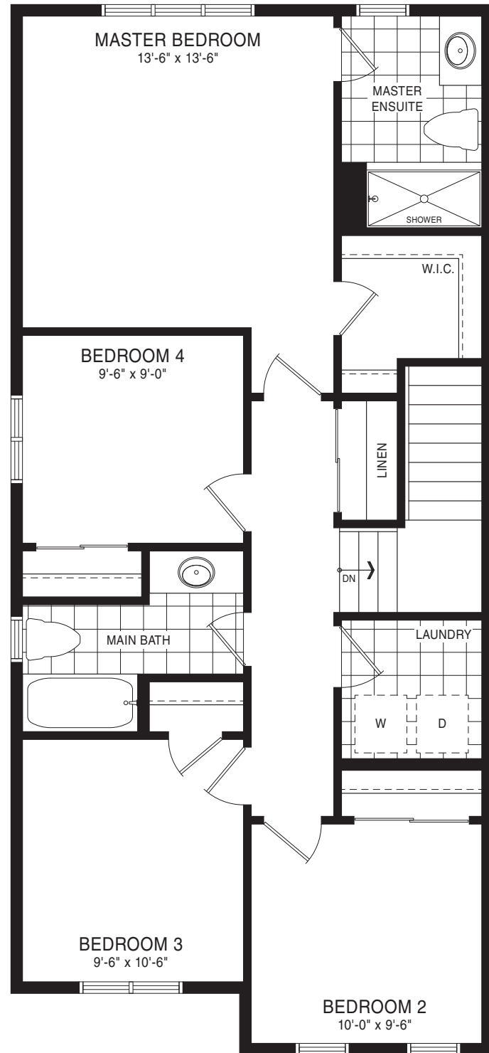
SECOND FLOOR PLAN STYLE A1
