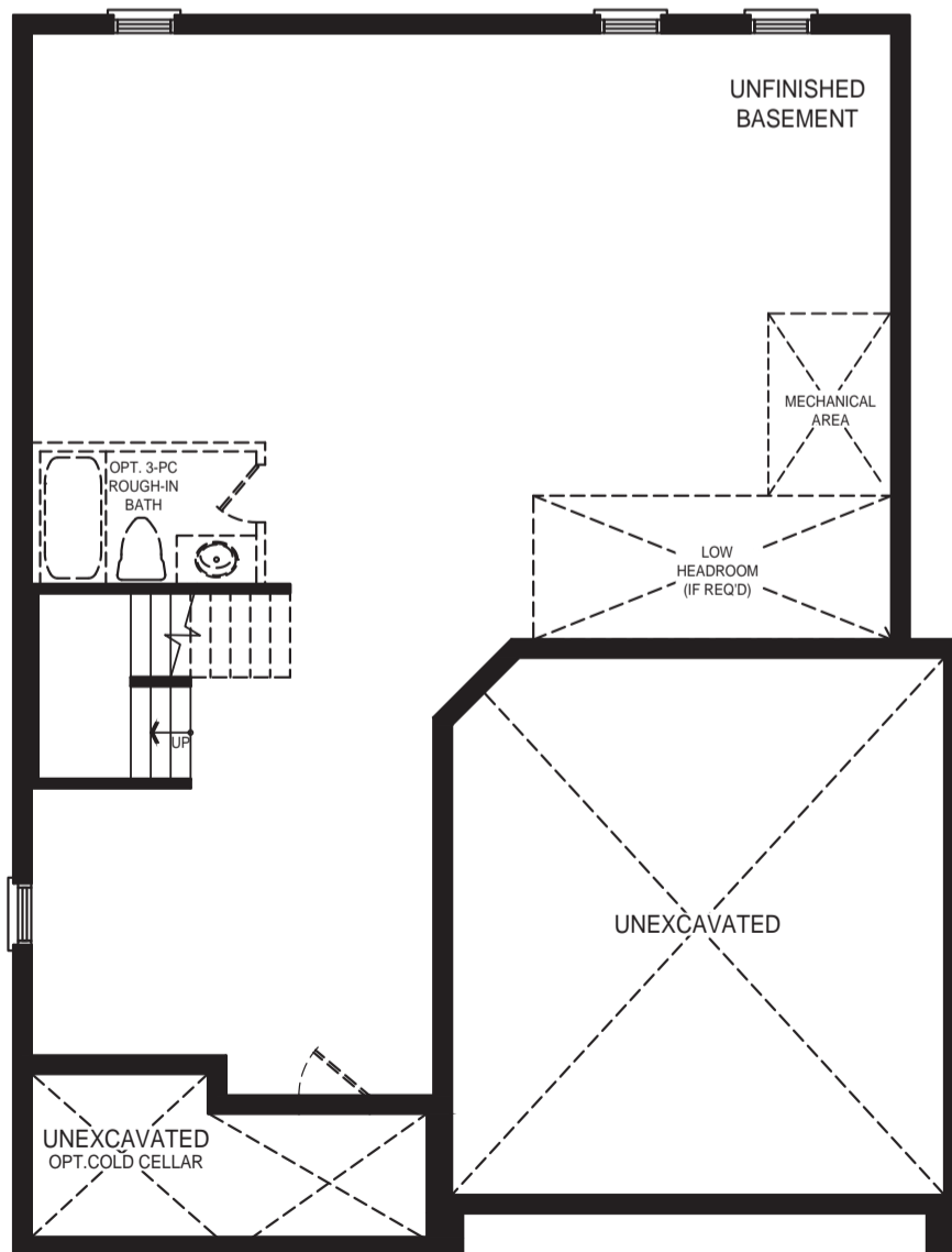
BASEMENT PLAN STYLE A
