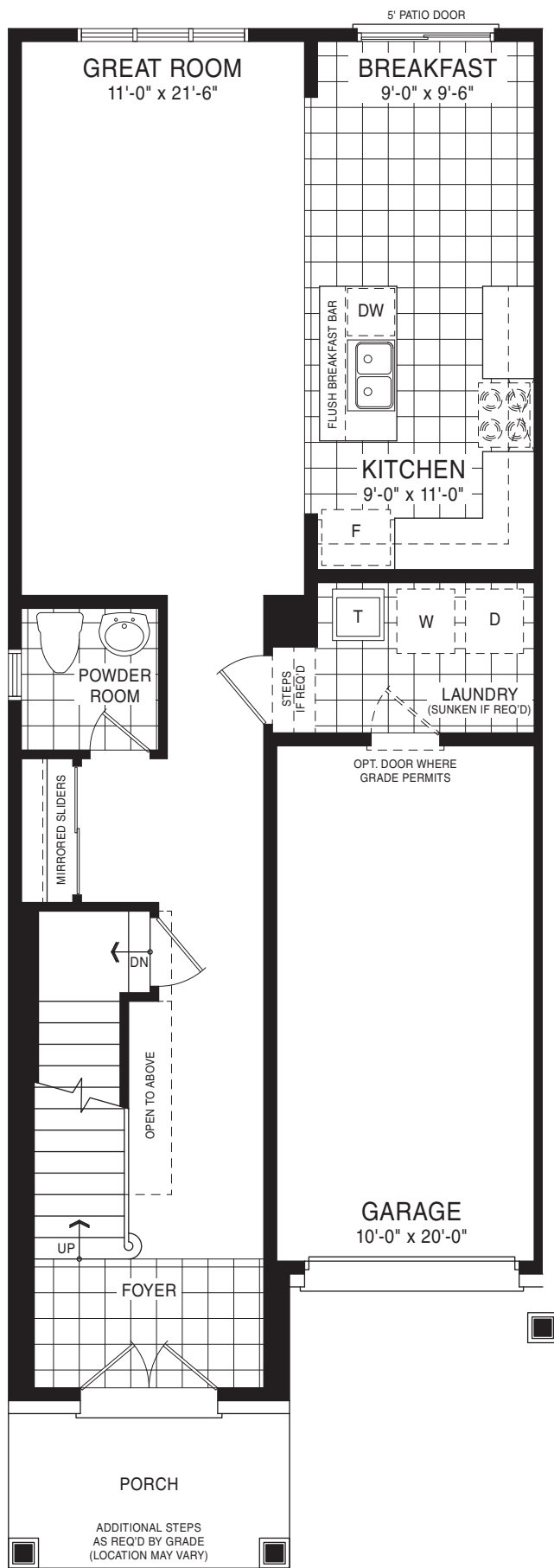
MAIN FLOOR PLAN STYLE A1
