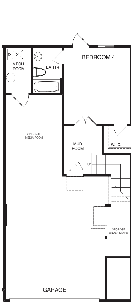
FIRST FLOOR PLAN ELEVATION A
