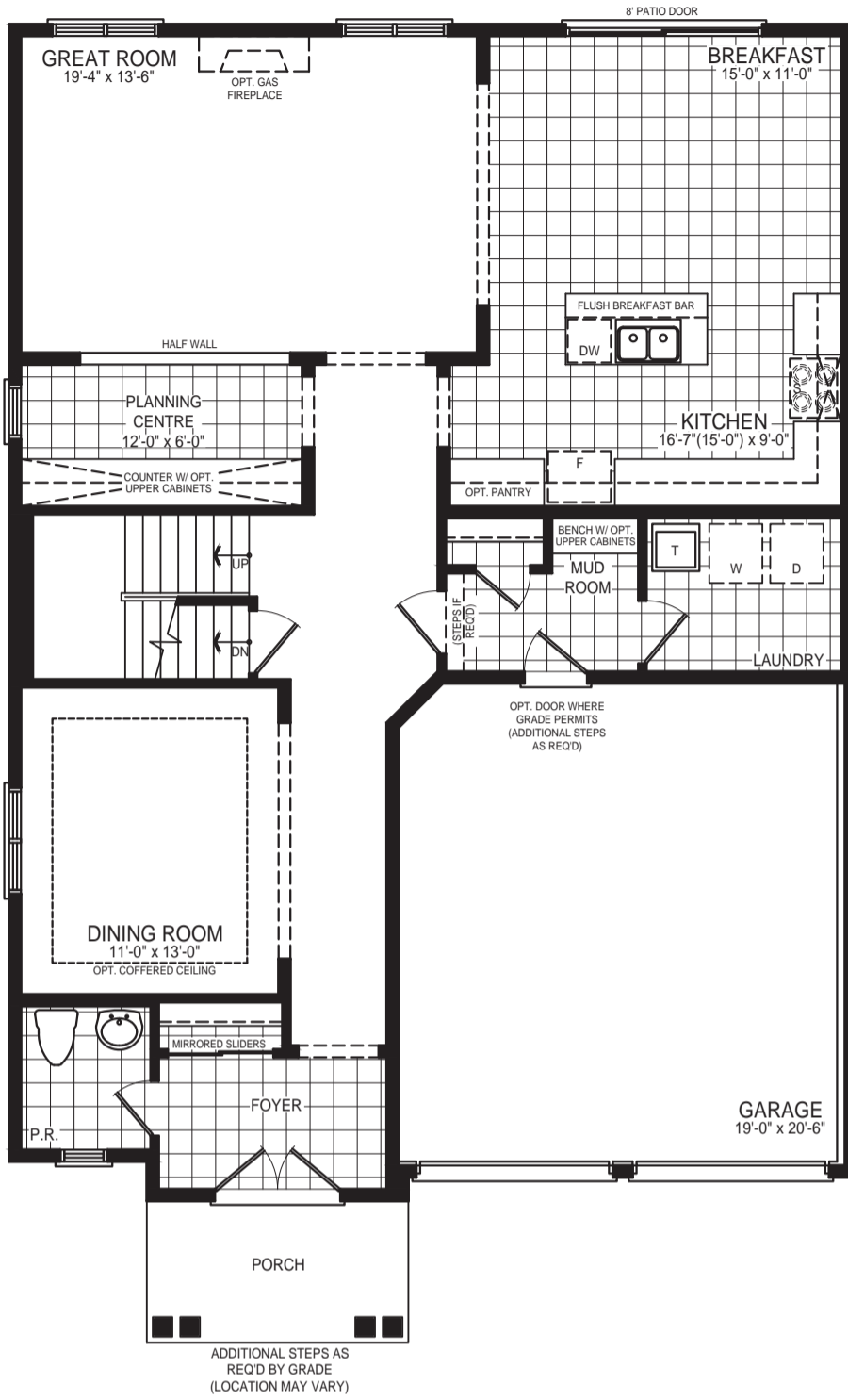
GROUND FLOOR PLAN STYLE A
