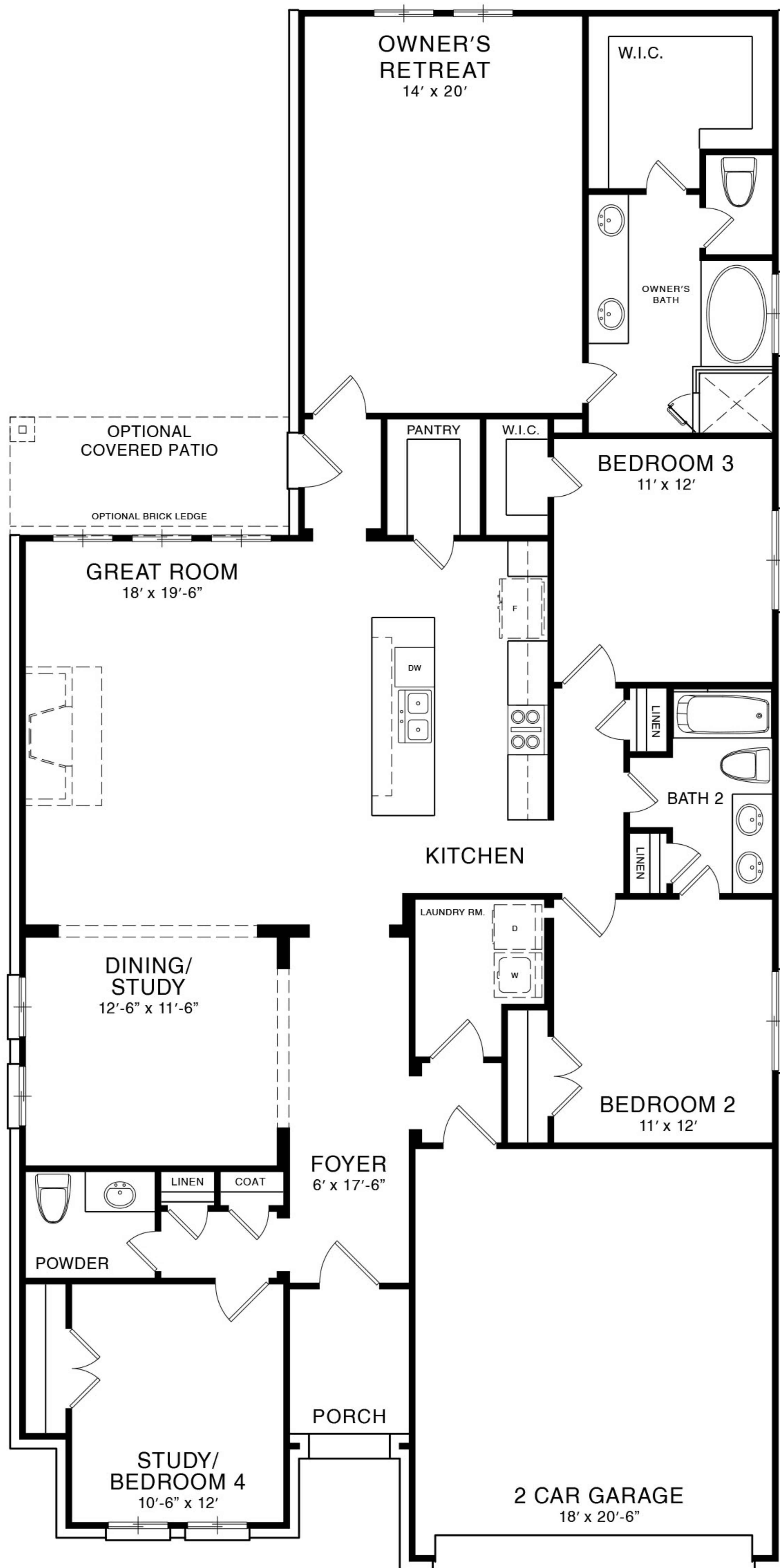
MAIN FLOOR PLAN STYLE A
