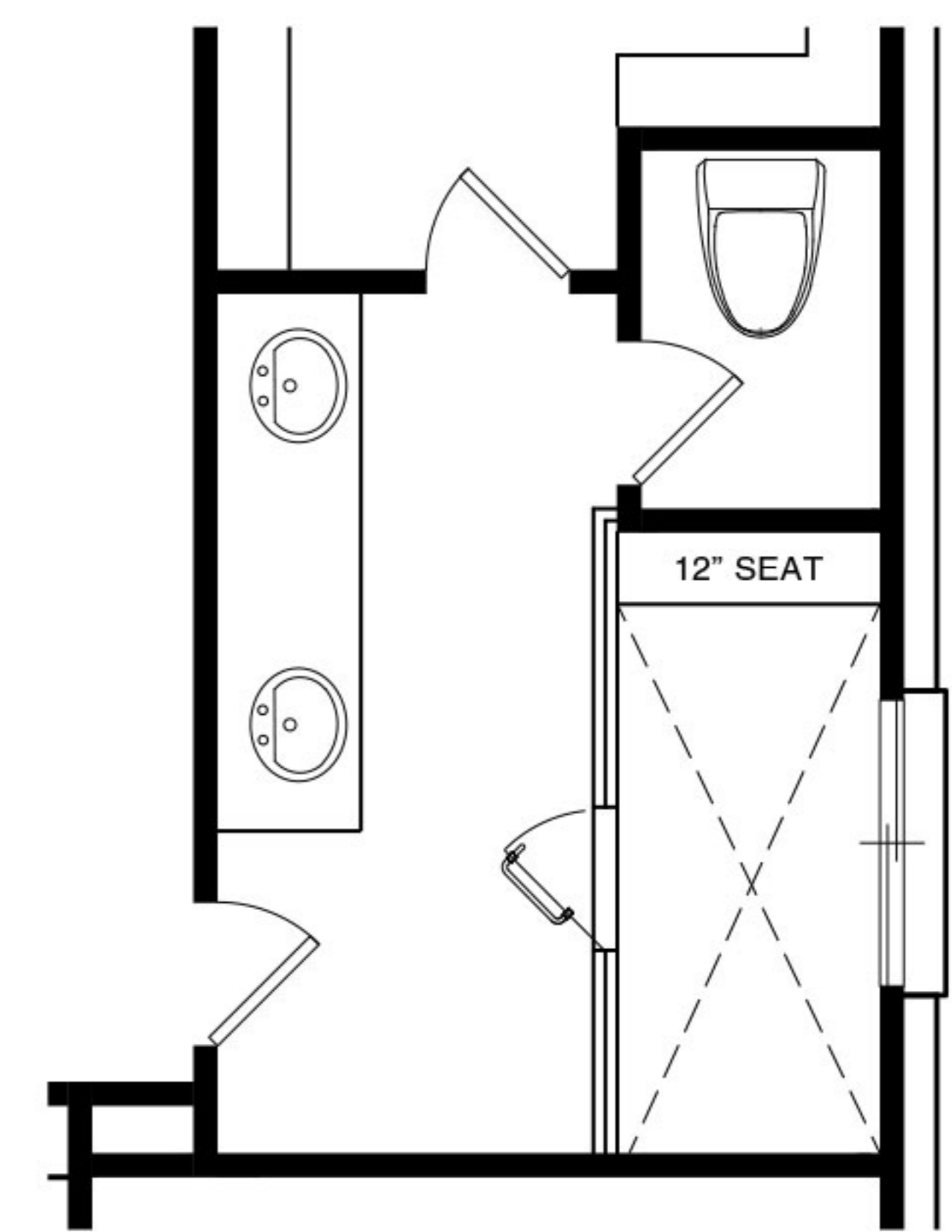
OPTIONAL WALK-IN SHOWER STYLE A
