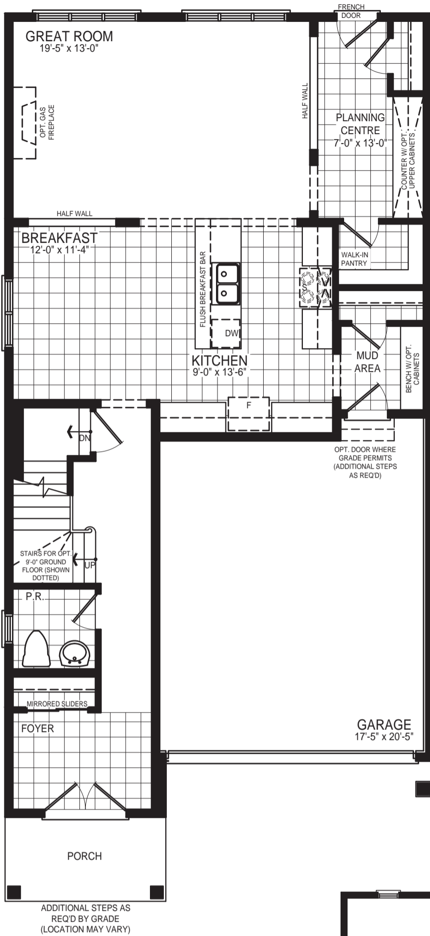
GROUND FLOOR PLAN STYLE A
