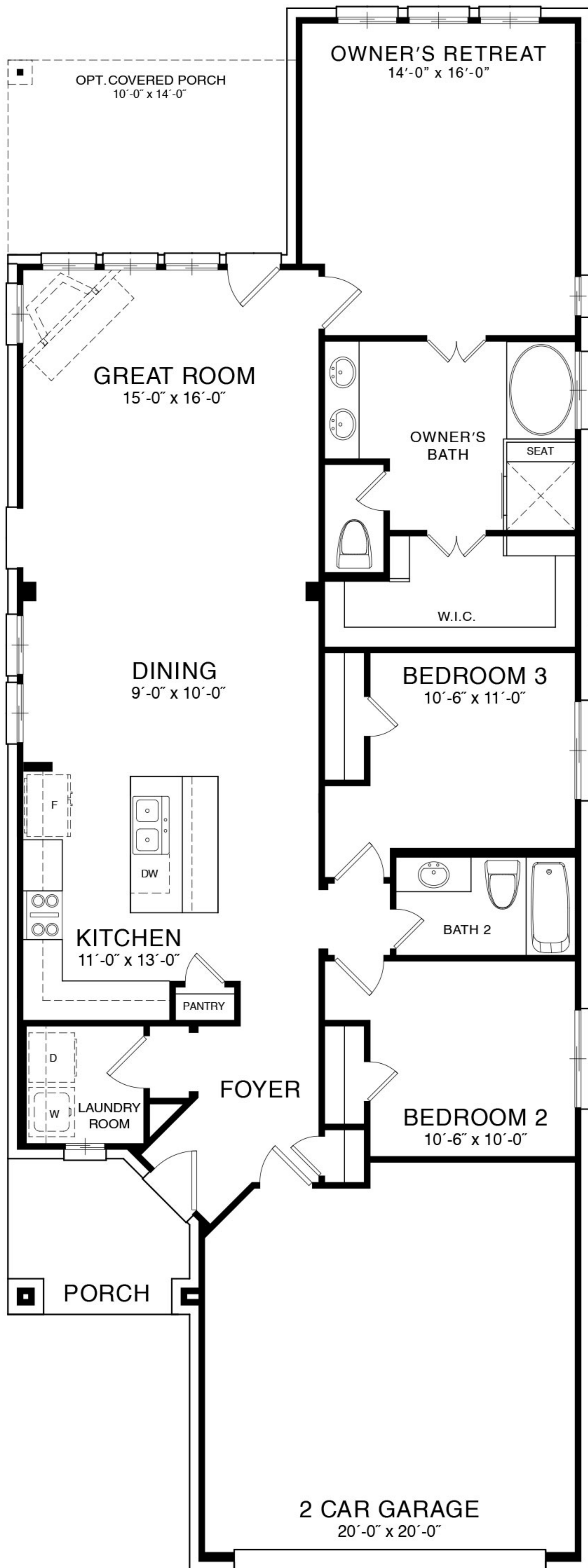
MAIN FLOOR PLAN STYLE A
