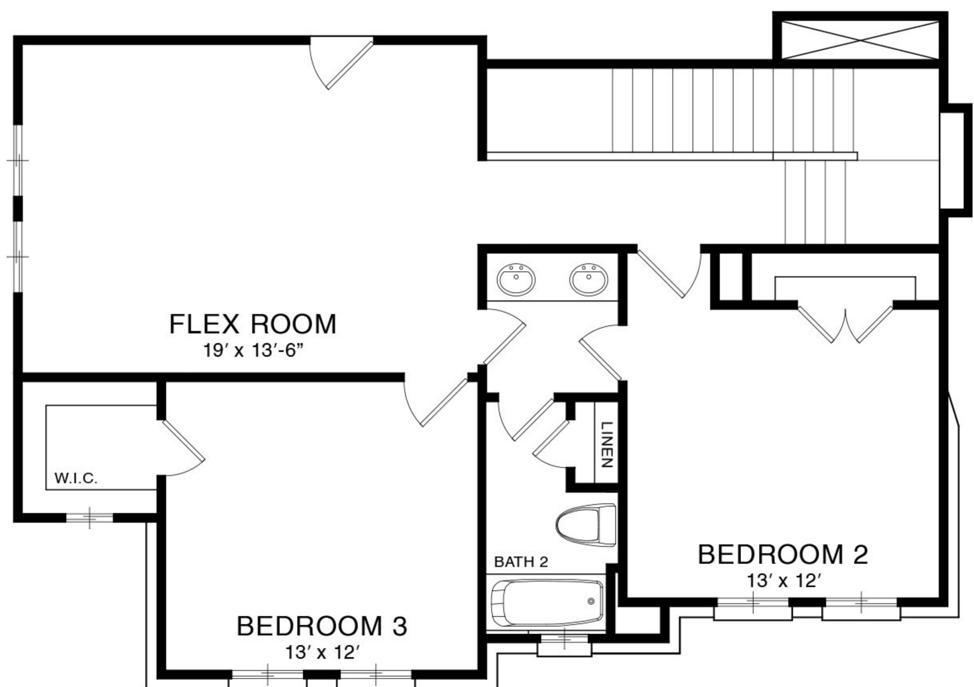
SECOND FLOOR PLAN STYLE A
