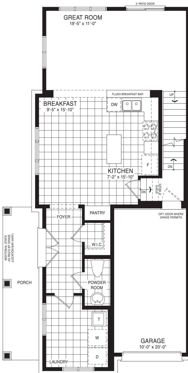
MAIN FLOOR PLAN STYLE A
