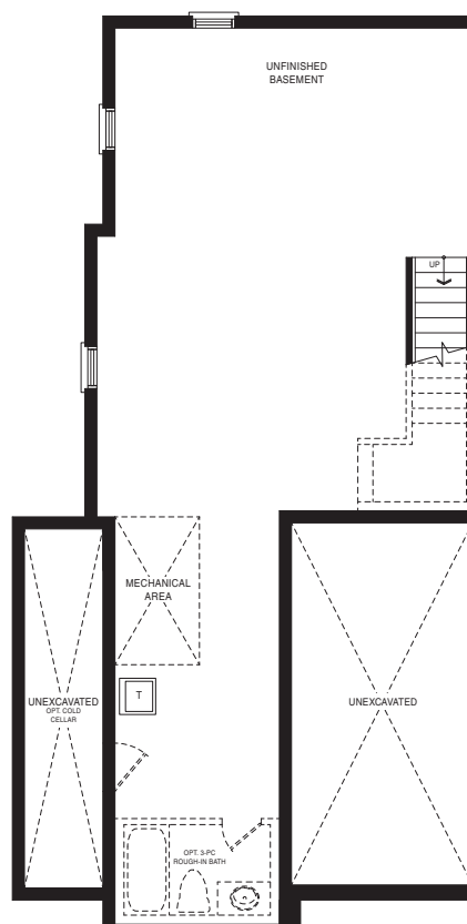
BASEMENT PLAN STYLE A
