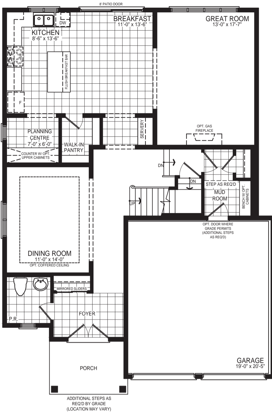
GROUND FLOOR PLAN STYLE A
